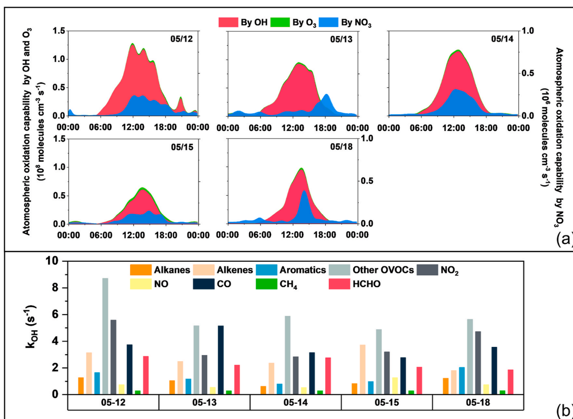
Fig. 4. (a) Simulated atmospheric oxidization capability in typical cases. (b) Breakdown of OH reactivity in each episode ( \text{s}^{-1} ).
