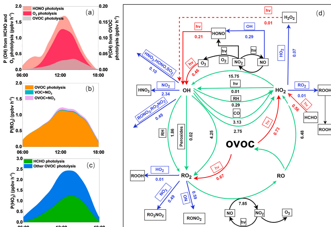
Fig. 5. Breakdown of average daytime production pathways of OH (a), RO_2 (b) and HO_2 (c). (d) Daytime average RO_x budget in 5 HCHO pollution cases. The unit is ppbv h^{-1} . The green, red, and blue lines indicate the recycling, primary production, and sink pathways of RO_x , respectively. (For interpretation of the references to colour in this figure legend, the reader is referred to the Web version of this article.)
