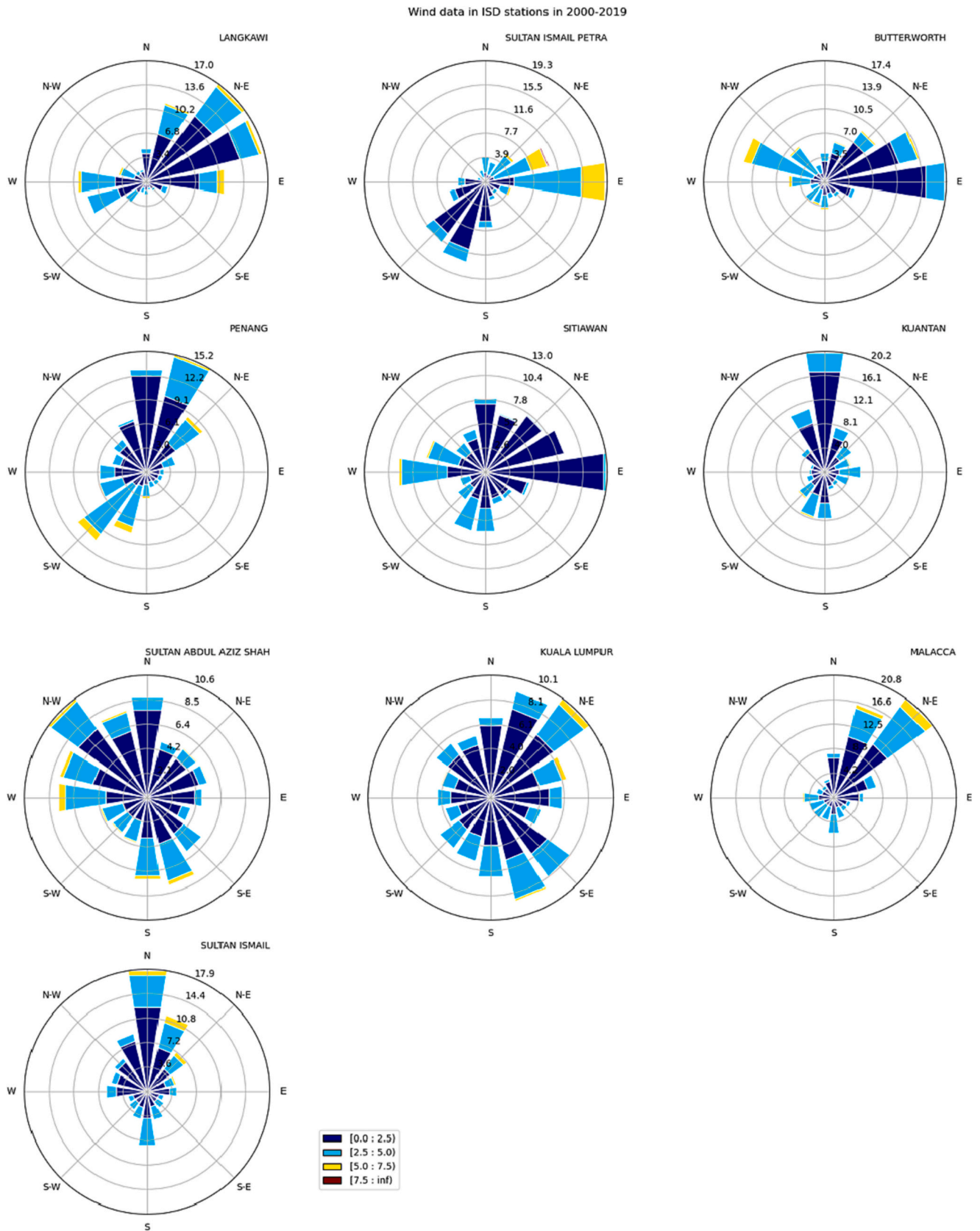
Fig. 5. Wind rose map of the surface hourly wind speed and wind direction from 10 general weather stations over the observation period.
