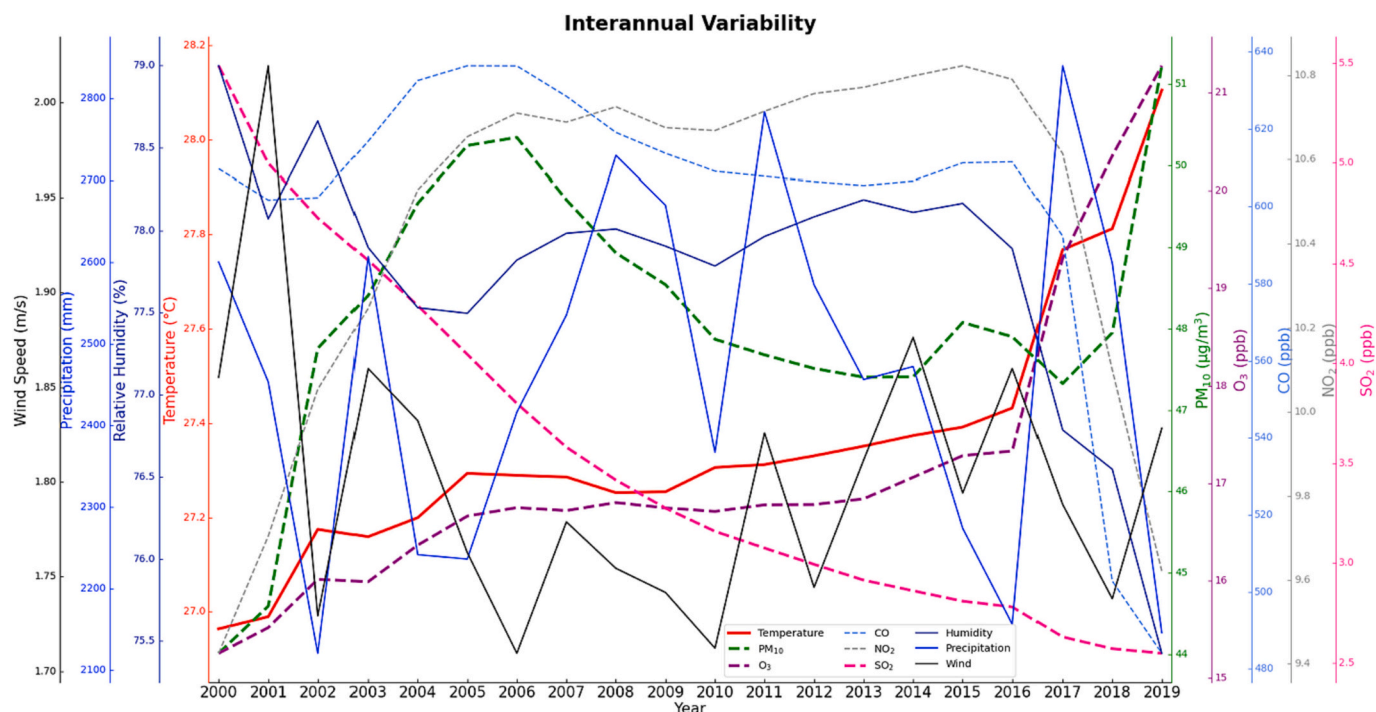
Fig. 2. Interannual variability of yearly climate (mean temperature, relative humidity, precipitation, and wind speed; solid lines) and air quality (PM 10 , O 3 , CO, NO 2 , and SO 2 ; dotted lines) over the observation period.
