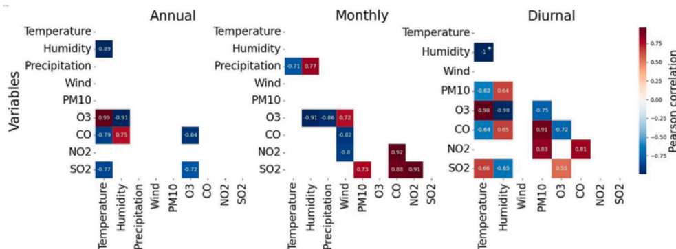
Fig. 9. Pearson correlation coefficients of the mean temperature, precipitation, relative humidity, wind speed, PM 10 , O 3 , CO, NO 2 , and SO 2 over the observation period. (Correlation values are shown only for those pairs of variables that passed the significance test at the 99 % confidence level.)
