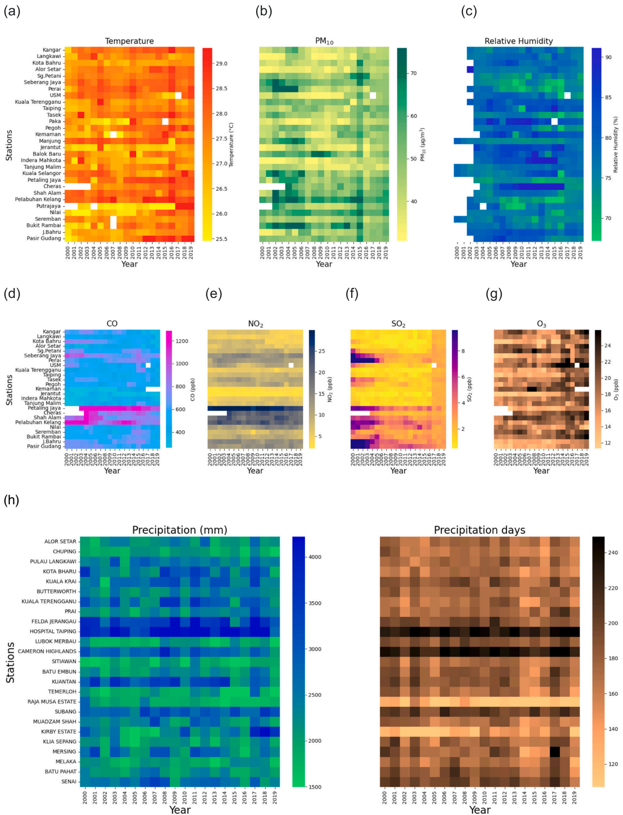
Fig. 3. (a) Yearly mean temperature, (b) PM 10 , (c) relative humidity, (d) CO, (e) NO 2 , (f) SO 2 , (g) O 3 , and (h) precipitation amount and days with precipitation from north (top) to south (bottom) over the observation period.
