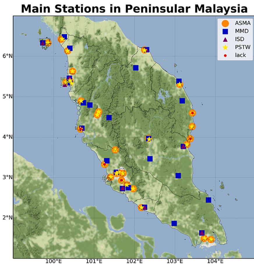
Fig. 1. Locations of the data used in this research, including continuous air quality monitoring system (CAQMS) stations from PSTW (yellow stars) and ASMA (orange circles), general stations for wind data from the ISD (purple triangles), and Malaysian meteorological department weather stations (blue squares). Note that stations in red circles lack air quality data concerning the concentrations of O_3 , CO, NO_2 , and SO_2 .
